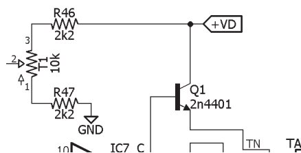
Prototype schematic with incorrect connection. BAD BEAN!
